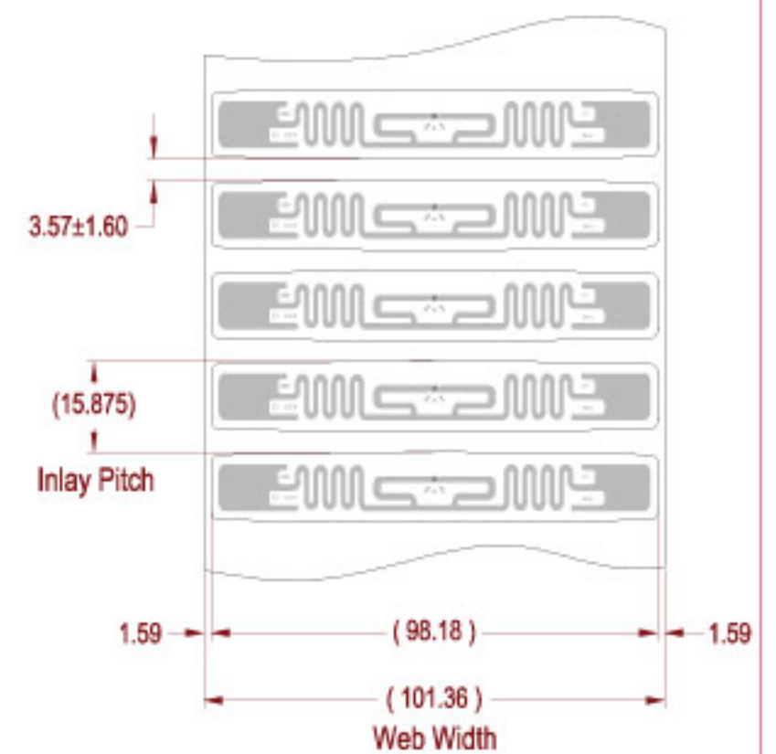
ALN-9640-FWRC / -FWRW (Clear / White Wet Inlay)
