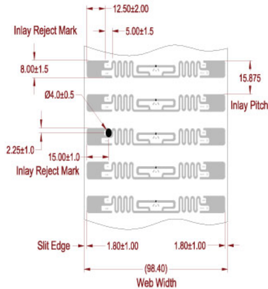
ALN-9640-FSR (Dry Slit Roll)
